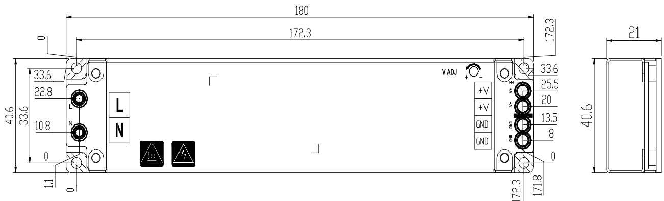
Dimensions and mounting holes - terminal coordinates
